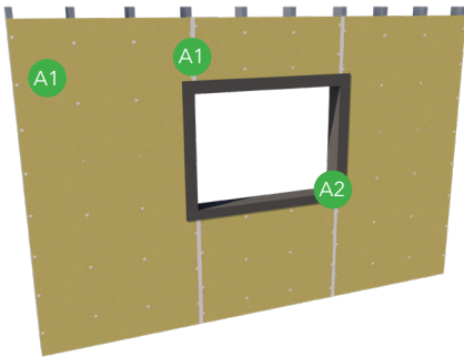
Permeable rough opening: VaproLiqui-Flash™
